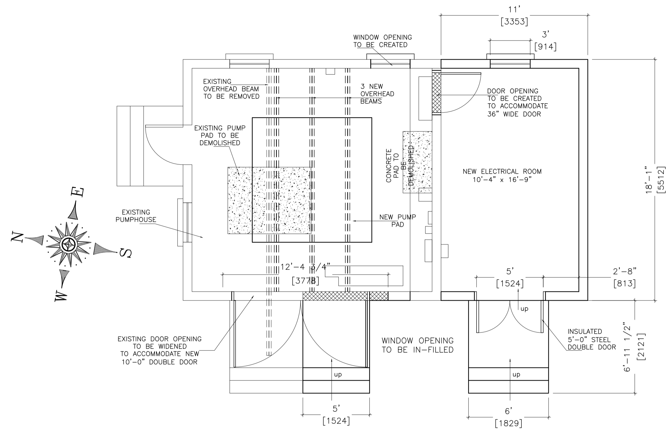
GENERAL ARRANGEMENT PLAN SCALE 1:50
