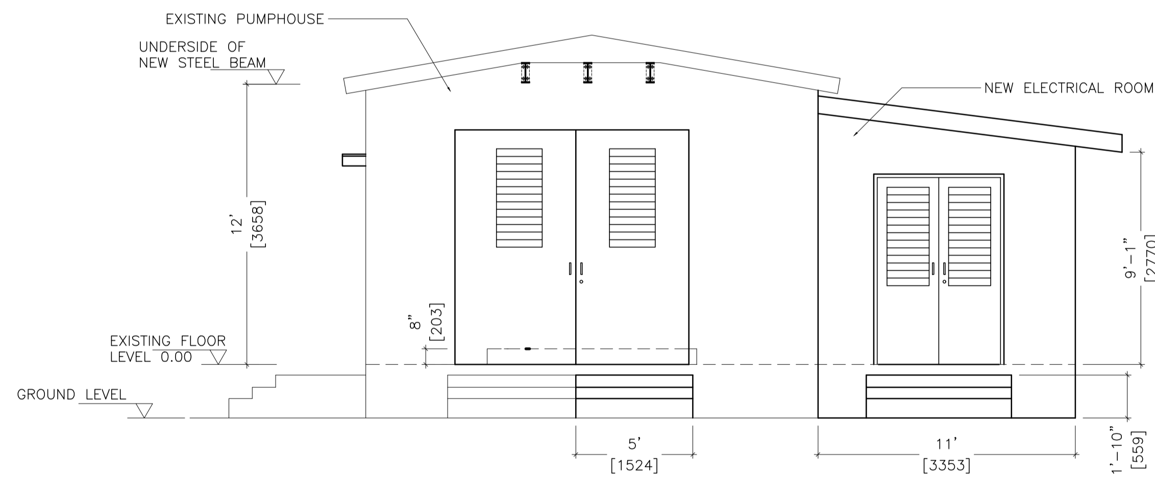
WEST ELEVATION SCALE 1:50
